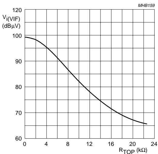
Fig.6 Typical tuner takeover point as a function of resistor R TOP .
