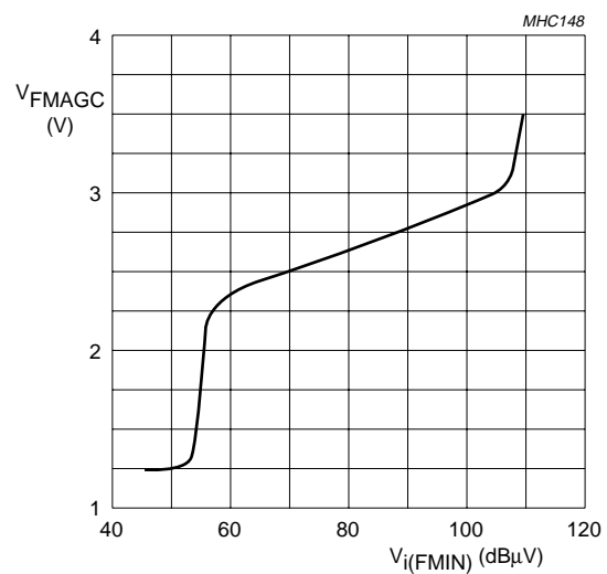
Fig.7 Typical FM-AGC characteristic.
